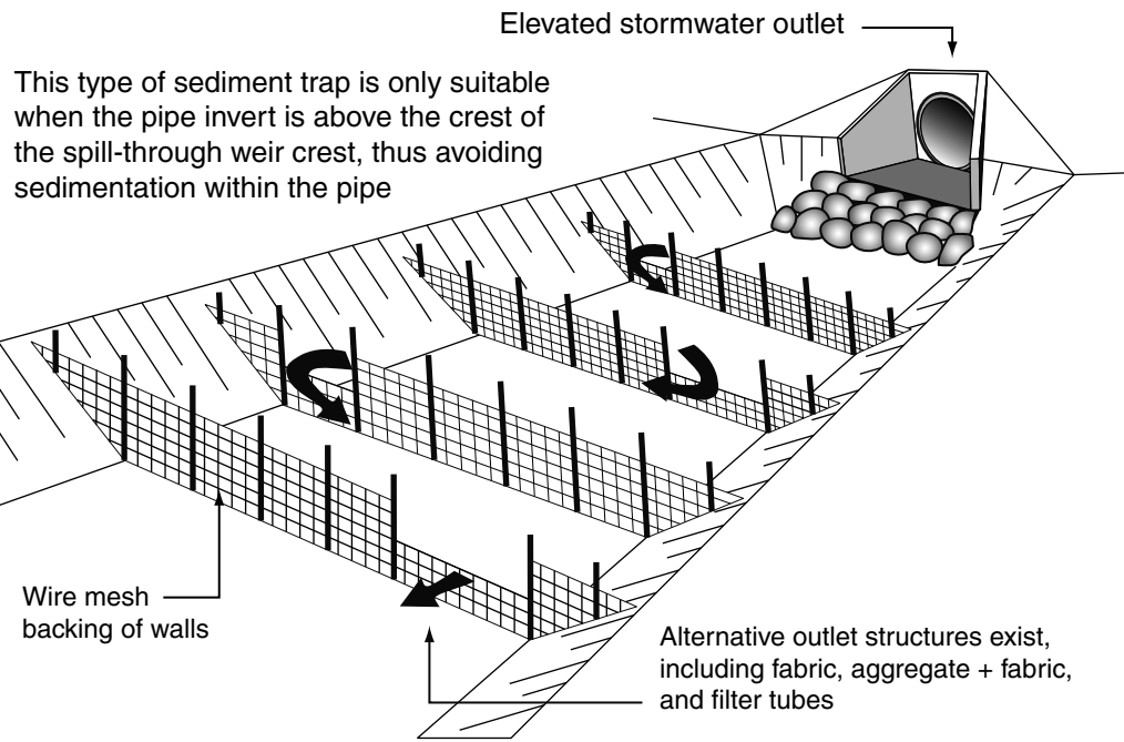
(a) Coarse sediment trap outlet system
