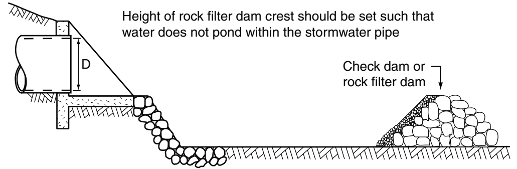
(c) Rock filter dam outlet sediment trap
