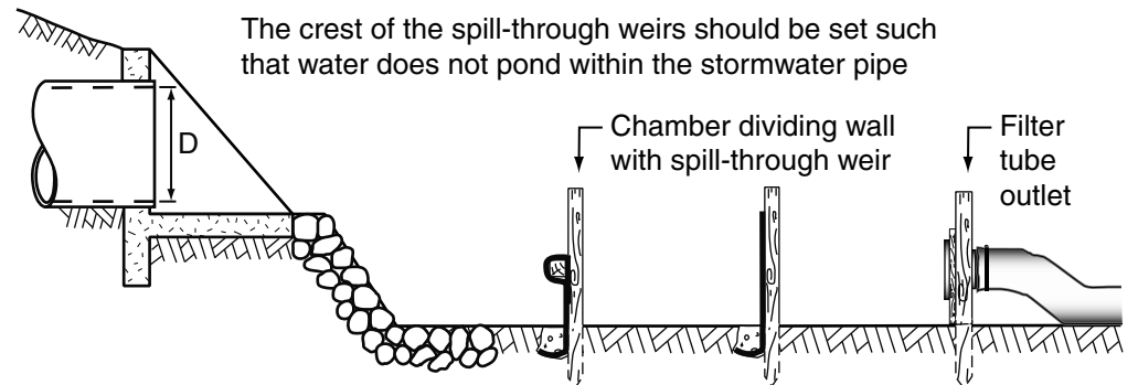
(e) Coarse sediment trap with filter pipe outlet
