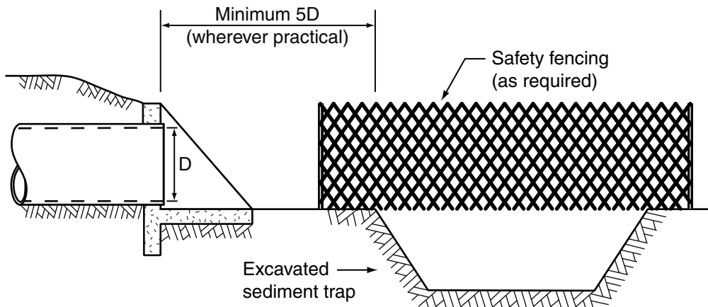
(b) Excavated sediment trap outlet system
