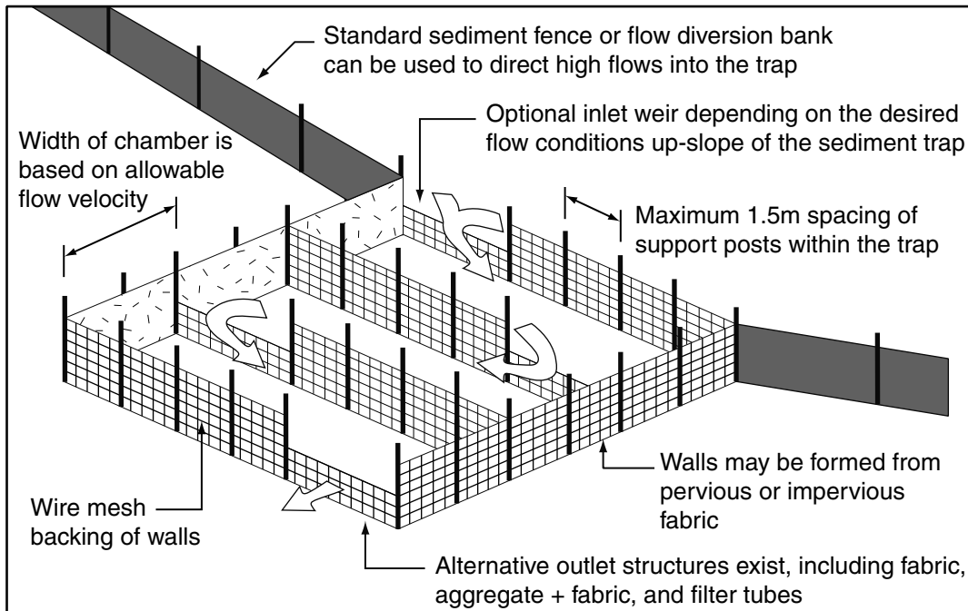
(a) Typical layout of a coarse sediment trap
