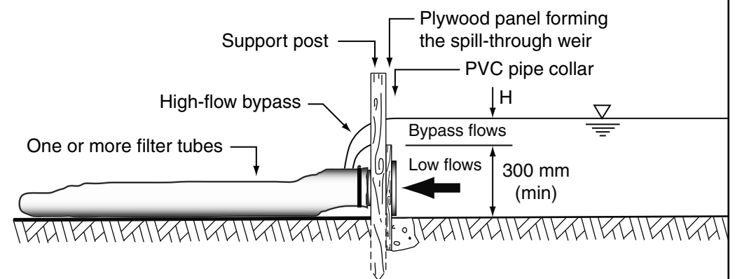
(e) Alternative outlet structure incorporating a filter tube
