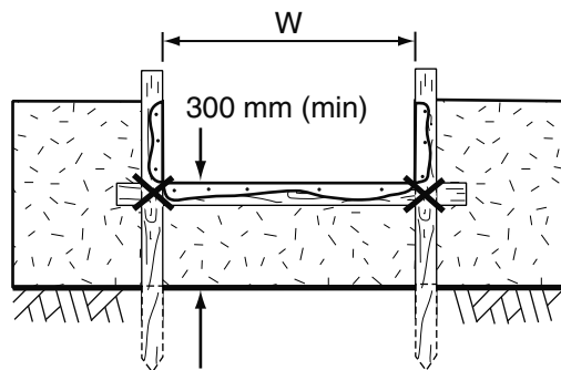
(c) Spill-through weir
