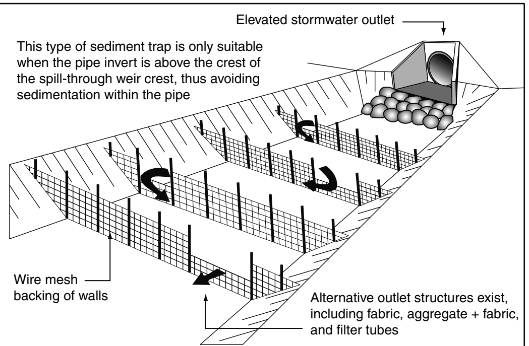
(b) Coarse sediment trap located at pipe outlet
