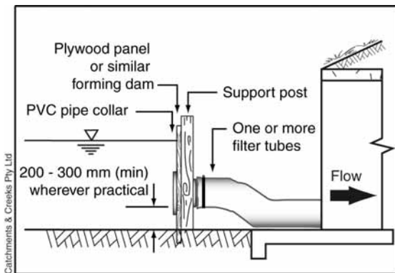
Figure 5 – Filter tube dam system
