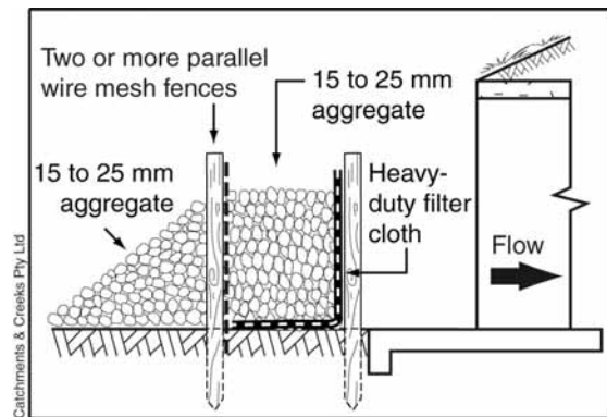
Figure 6 – Sediment weir system
