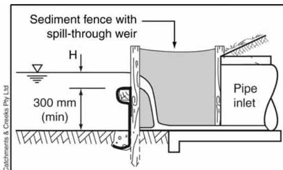
Figure 7 – Sediment fence system
