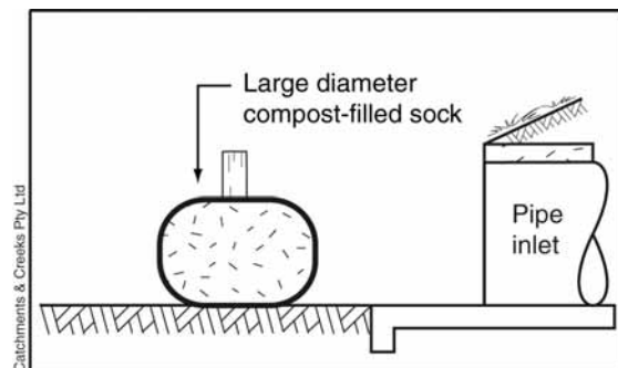
Figure 8 – Compost-filled filter sock
